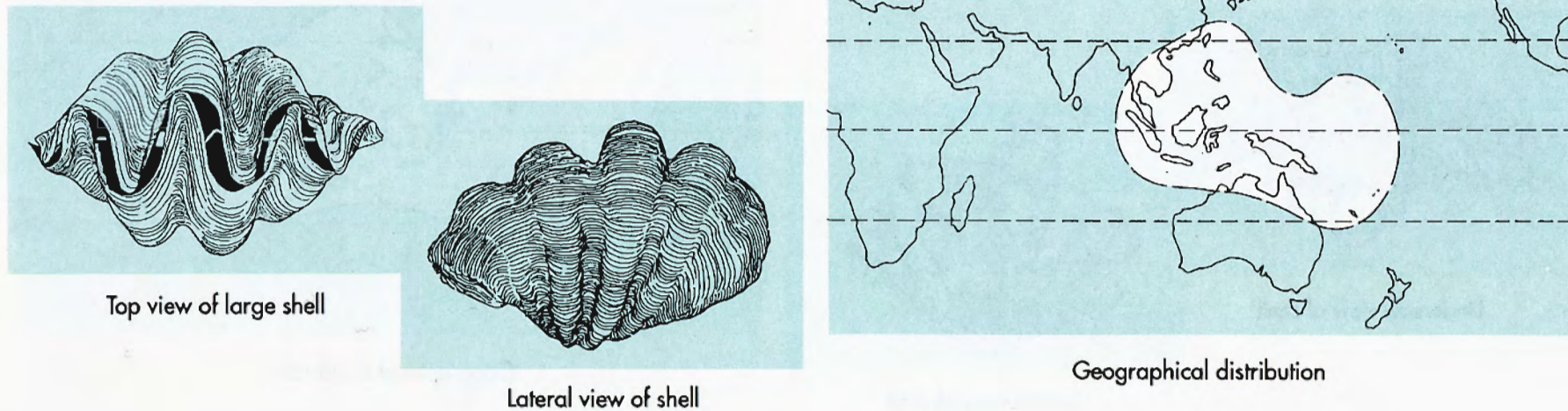
Figure 1.2 Tridacna gigas
