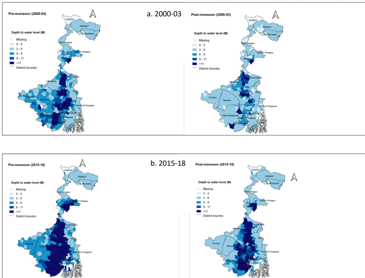
Figure 19: Pre and post monsoon water levels in West Bengal, 2000-03 and 2015-18 Source: Data from SWID
