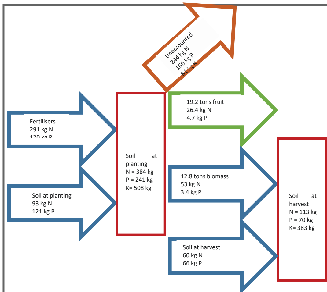
Figure 44. NPK inputs and outputs in a watermelon trial, Fahefa soil type. Blue arrows soil inputs, grower arrow exports, orange arrows losses and red boxes the soil.
