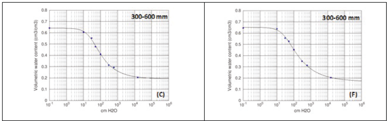
Figure 22 Soil water retention characteristics of the Nu'u 1 (A-C) and Faleālili (D-F) sites for three different depth intervals. Blue dots show measured data points and black solid lines denotes the fitted van Genuchten (1980) model. Soil bulk density and the van Genuchten model parameters are shown in Table 3.
