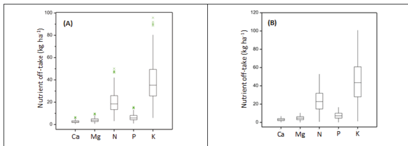
Figure 27. Estimated nutrient off-take in taro corms at Nu'u 1 (A) and Faleālili (B) in 2018-2019. Data shown in boxplots are as described in the caption of Figure 5.
