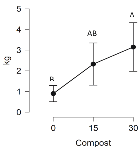
Figure 18 Influence compost (%) on cabbage yield. Compost and irrigation trial Kiribati. Significant difference at the p \leq 0.05 .
