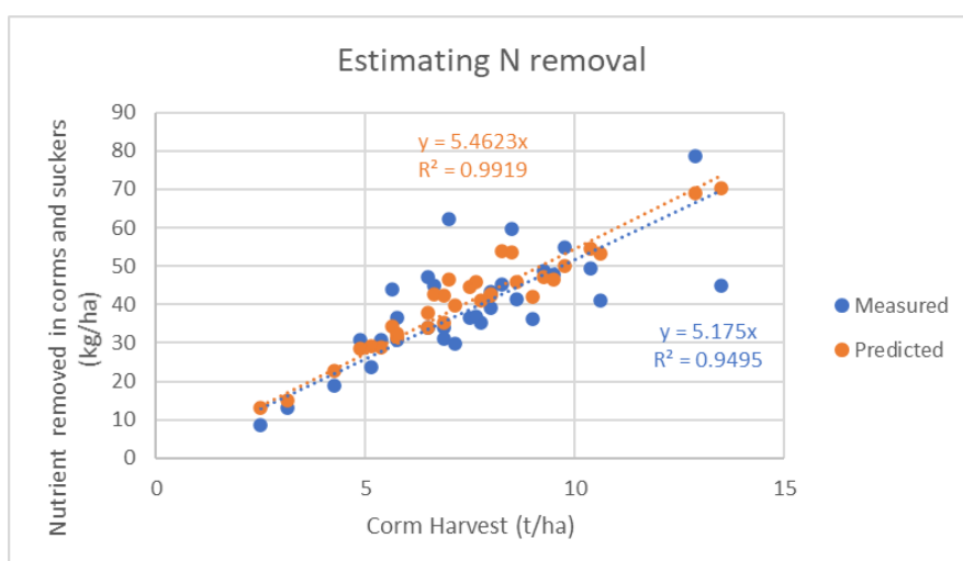
Figure 38. Estimation of N removal from the taro field using literature values (Bradbury and Holloway 1988) and measured values from the field trials.
