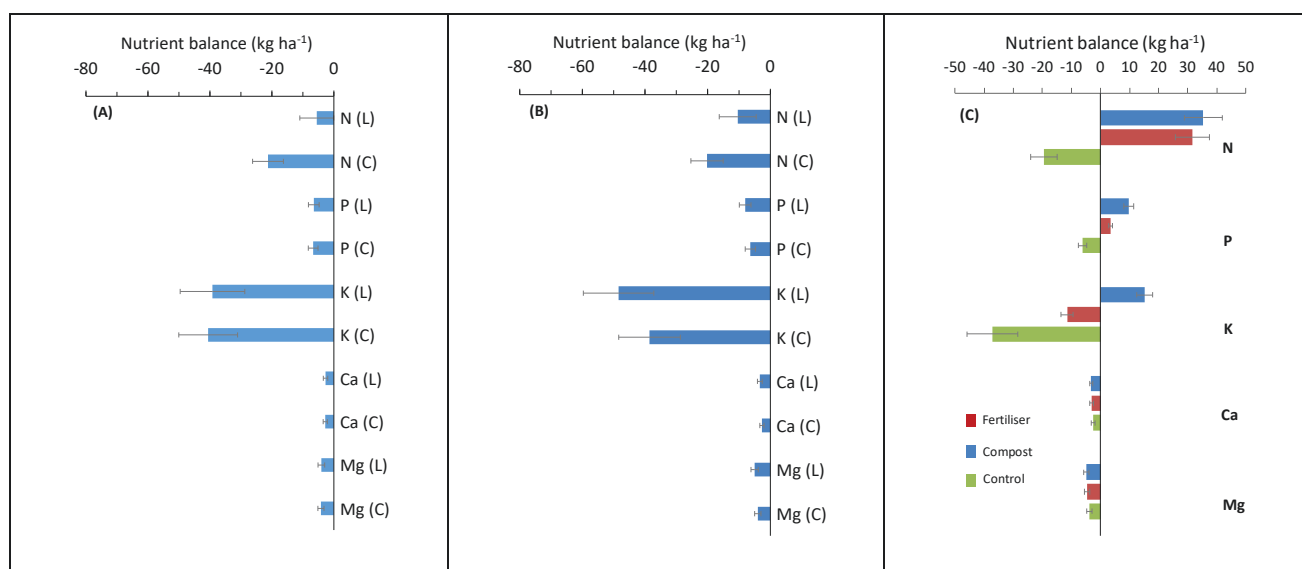
Figure 29 . Estimated field-scale (macro) nutrient balance at three experimental sites as affected by nutrient management practice. From left to right, (A): Nu'u 1 (2018-2019), (B): Faleālili (2018-2019), and (C): Nu'u 2 (2020-2021). In Figures (A) and (B), the letters (L) and (C) following the nutrient symbol denote 'legume' intercropping and 'control', respectively. In Figure (C), 'fertiliser' is NPK+S (12:8:15+3, commercially known as Blaukorn Classic®) and 'compost' is composted poultry manure (>¾ by weight).
