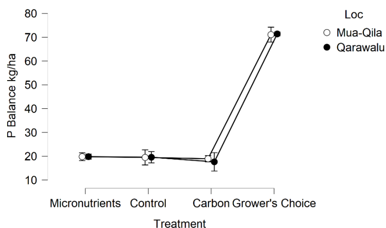
Figure 37. Phosphorus balance in each field Phase 2 field trial, Taveuni 2019-2020
