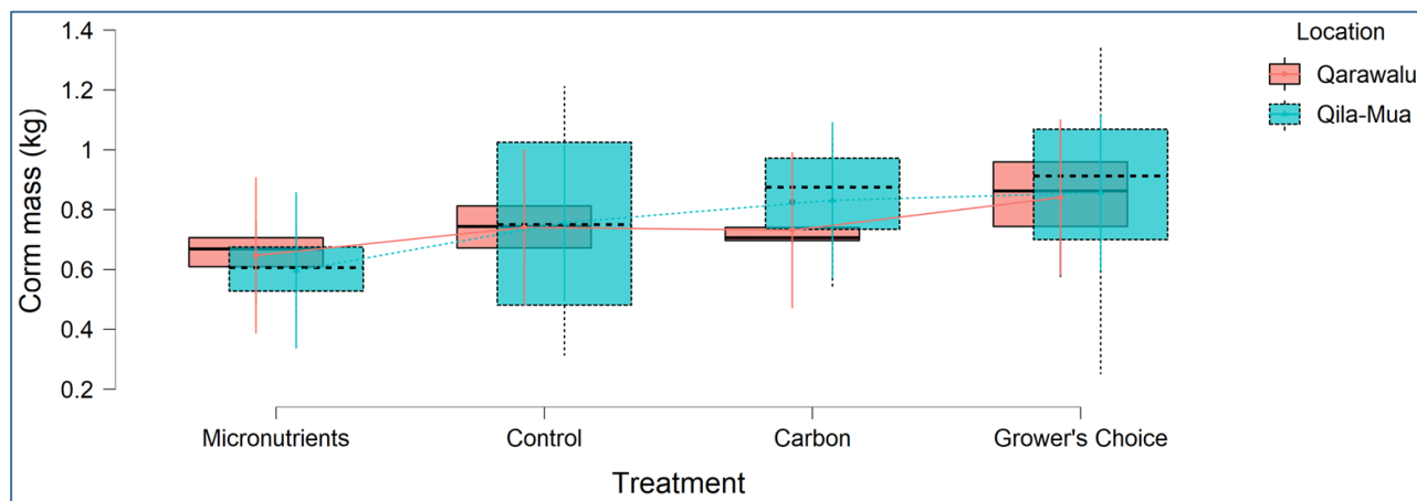
Figure 33. Mean taro yield Phase 2 Taveuni field trial.
