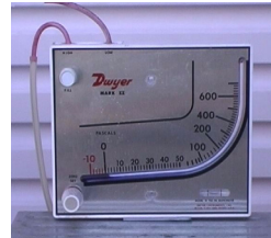
Inclined manometer
