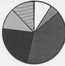
Fruit Program
