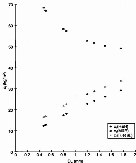
Figure 5. Comparison of the values of c_t calculated for the three versions of GUEST for erosion events on the bare 10% slope plot at ViSCA, when the soil surface was unrilled (plane geometry). Symbols are: ◆, Hairsine and Rose (1992a, b); ■, Misra and Rose (1992); ▲, GUEST+.
