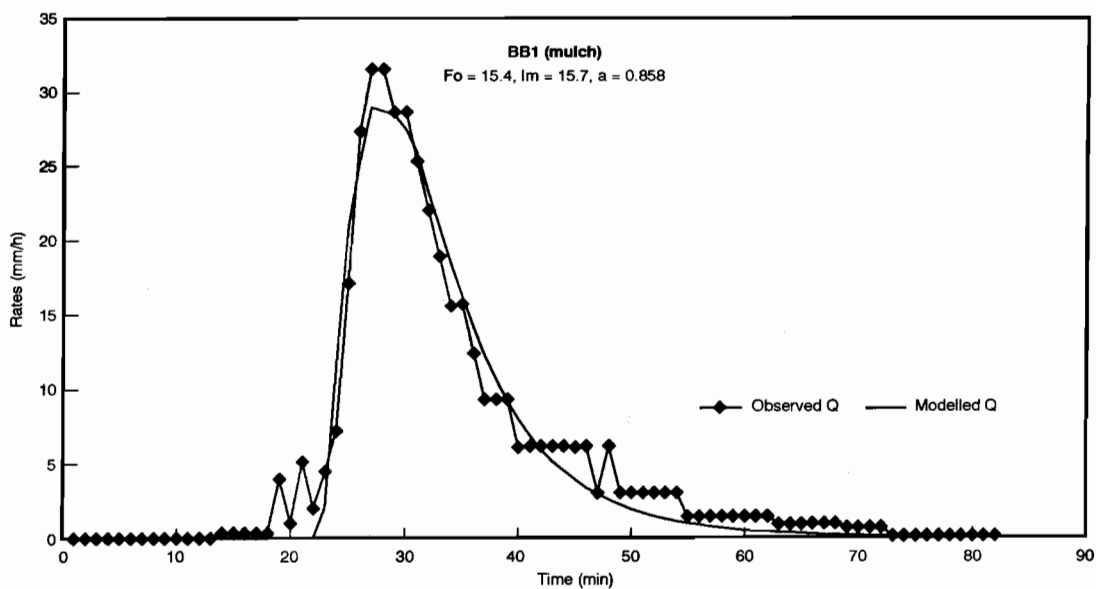
Figure 2c. Observed and modelled hydrographs at 1 minute intervals: event 22/02/93, BB2 conventional at Goomboorian.
