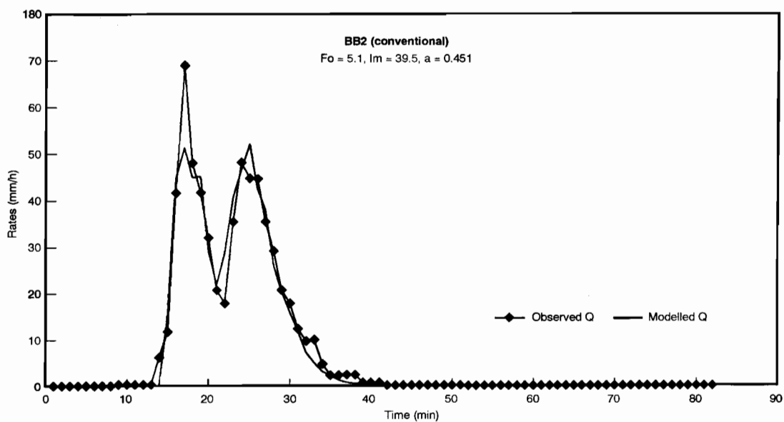
Figure 2b. Observed and modelled hydrographs at 1 minute intervals: event 22/03/93, BB1 (mulch) at Goomboorian ( E = 0.96 ).
