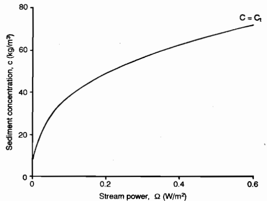
Figure 2. Illustrating the form of variation with stream-power in sediment concentration at the transport limit, c_t , for sheet flow.
