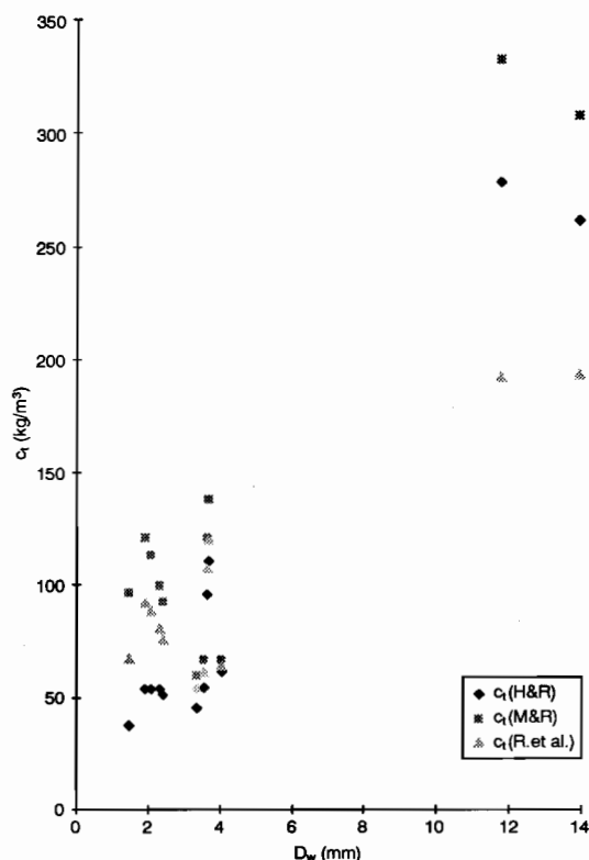
Figure 9. Comparison of the values of c_i calculated for the three versions of GUEST for erosion events on the Imlil, Queensland, pineapple plots, where flow is in the trapezoidal channels produced for pineapple culture. Symbols are: ♦, Hairsine and Rose (1992a, b); ■, Misra and Rose (1992); ▲, GUEST+.
