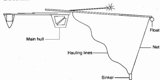
Fig. 30. The experimental baitfishing set-up of the 'PNG 11' outrigger canoe trialled in Butaritari.
