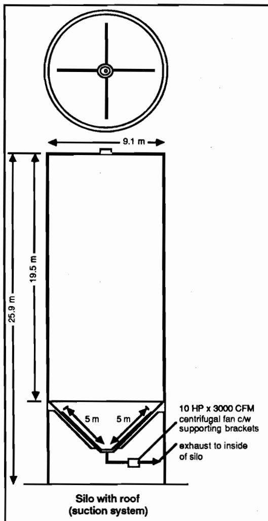
Fig. 1. Configuration of LPN aerated concrete silos fitted with roofs.
