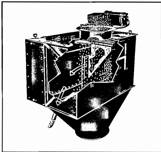
Fig. 27. Automatic cross-cut grain sample collector.
