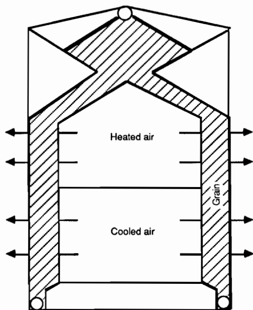
Cross flow dryer
