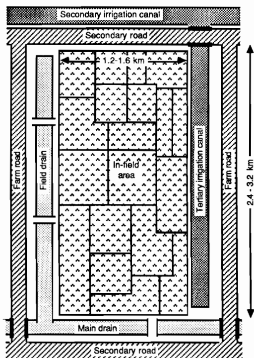
Fig. 3. Schematic representation of the layout of an irrigation unit in the Muda Agricultural Development Area in north-western Malaysia.
