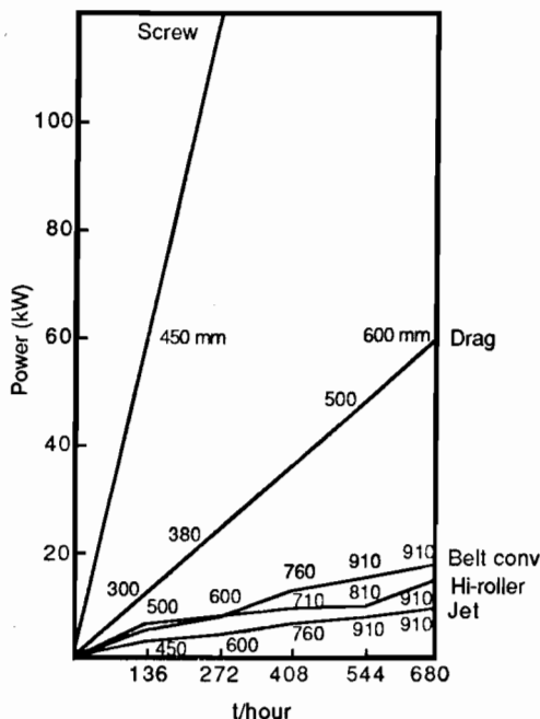
Fig. 14. Relative power requirements of different types of grain conveying systems.
