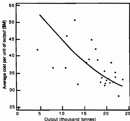
Fig. 1. Drying cost curve for paddy, relating drying output and average cost per unit of output.
