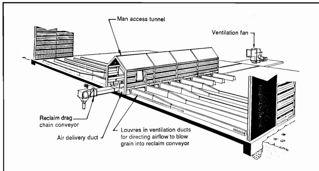
Fig. 6. Ventilation system for reclaiming grain from flat-bottomed storages.
