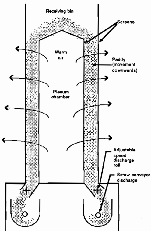
Fig. 2. Schematic drawing of air and paddy flow in a non-mixing columnar dryer.
