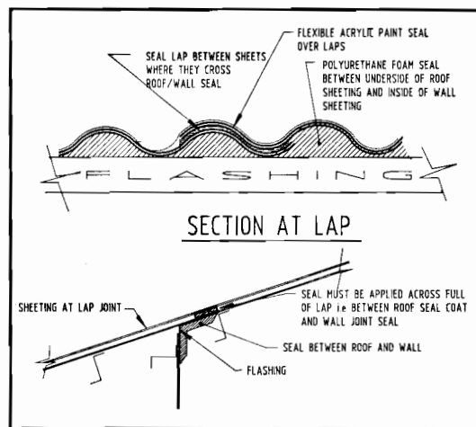
Fig. 19. Detail of lap joint sealing for a grain store.
