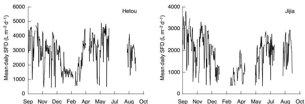
Figure 3. Seasonal variation in sap flux density in Eucalyptus urophylla at Hetou and Jijia, 1999–2000. Periods of missing data reflect failure of one or more instruments due to lightning or other causes.
