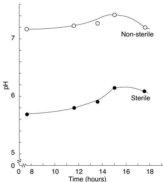
Figure 6. Fluctuation in pH at different times of the day under sterile and non-sterile conditions.
