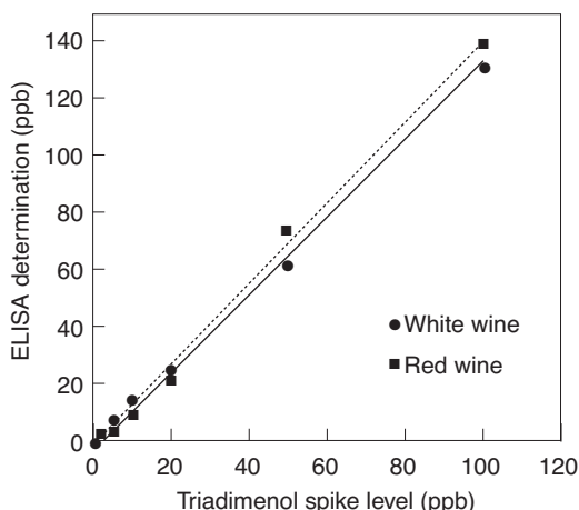
Figure 3. Recovery of spikes of triadimenol in red or white wine
