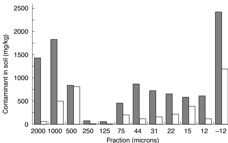
Figure 1. Concentrations of DDT and arsenic in various particle size classes of sandy soil following soil washing.
