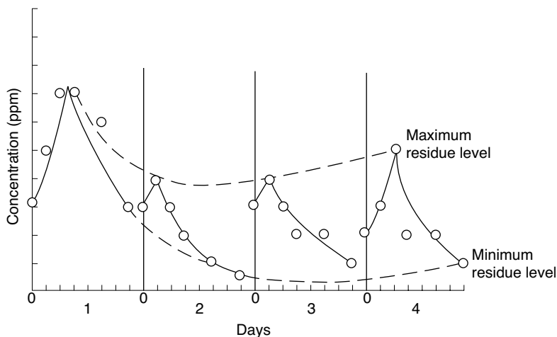
Figure 5. Levels of carbofuran in water following periodic application
