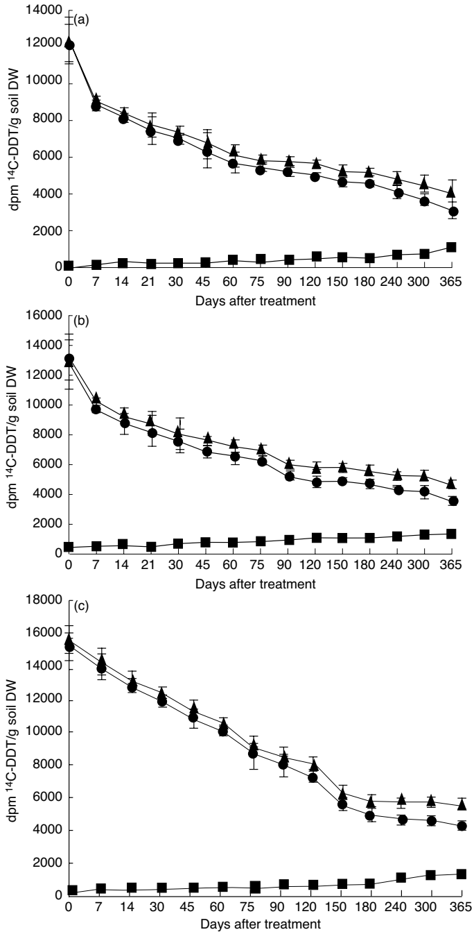
Figure 1. Dissipation of DDT from soil in (a) summer, (b) monsoon, and (c) winter: ●, extractable residues; ■, bound residues; ▲, total residues.
