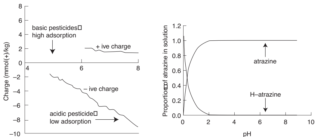
Figure 4. Effect of pH on dissociation of atrazine in relation to surface charge characteristics
