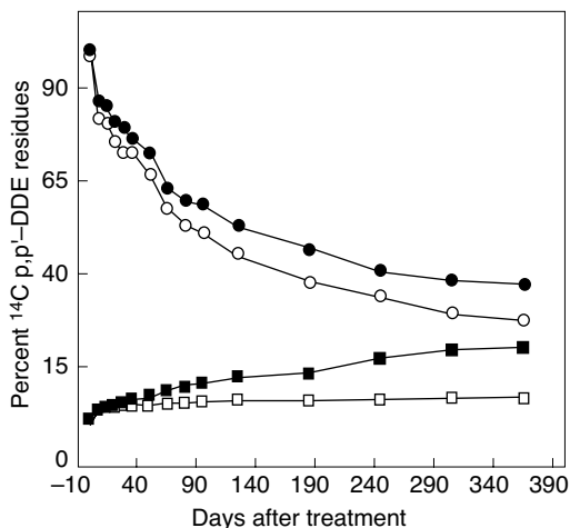
Figure 8. Persistence of ^{14}\text{C} and unlabelled DDE in field soil. Key: ●, total residues; ○, extractable residues; □, bound residues; ■, proportion of bound residues in total residues.
