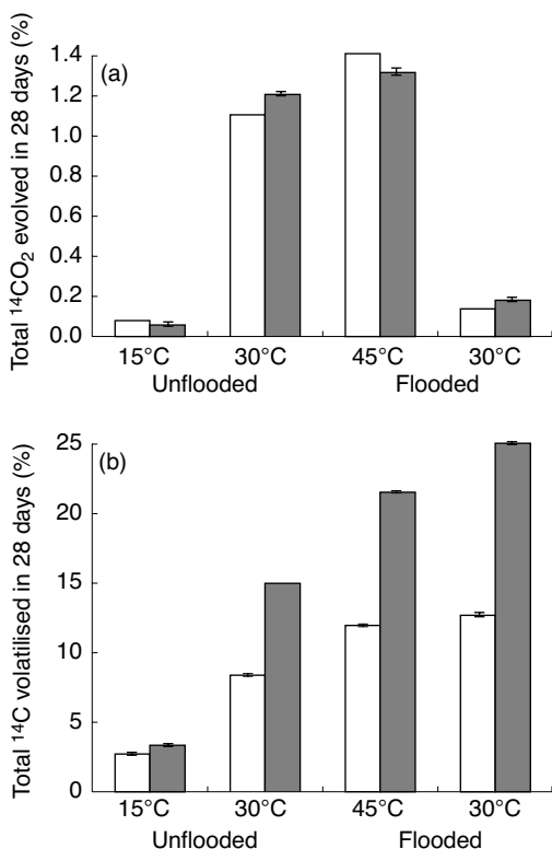
Figure 5. (a) Total 14 CO 2 released from soils treated with 14 C DDT (unshaded bars) or 14 C γ-HCH (shaded bars) at different temperatures. (b) Total 14 C volatilised from soils treated with 14 C DDT or 14 C γ-HCH at different temperatures
