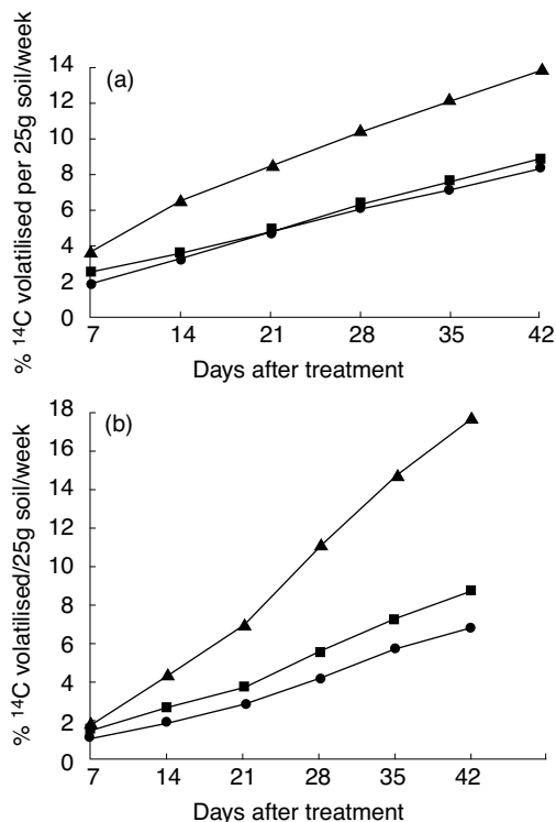
Figure 7. Cumulative percent volatilisation of 14 C DDT from (a) unflooded and (b) flooded soils exposed to solar radiation. Key: ▲, soil held in quartz tubes; ■, soil held in glass tubes; ●, soil held in dark tubes.
