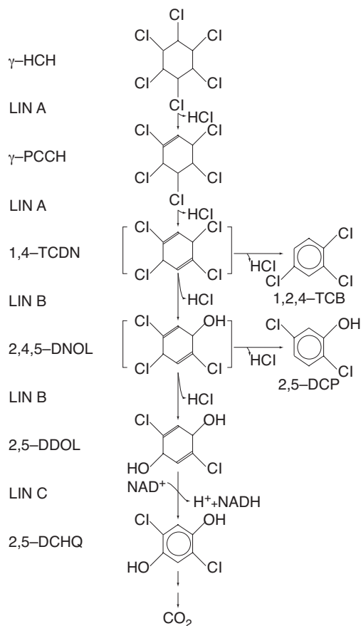
Figure 3. Proposed pathway of aerobic metabolism of \gamma -HCH by Sphingomonas paucimobilis .
