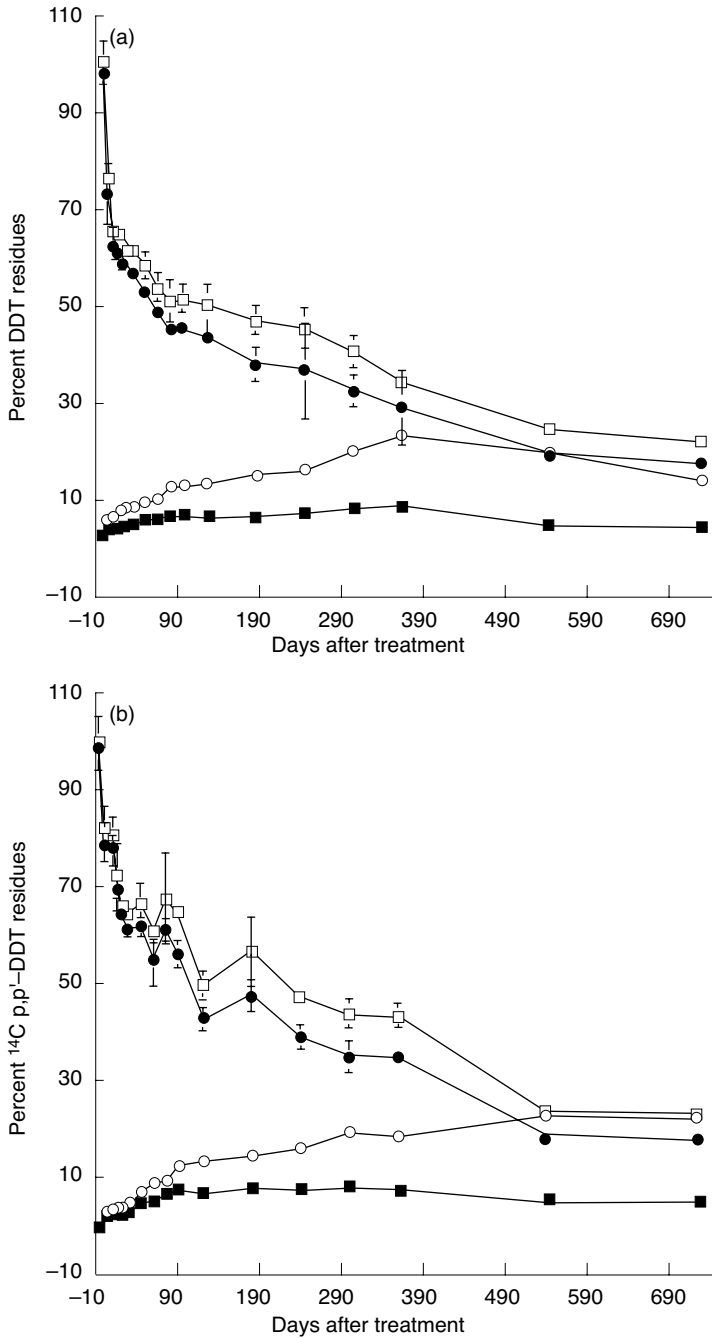
Figure 2. Persistence of 14 C and unlabelled DDT in field soil: (a) first experiment; (b) second experiment. Key: □, total residues; ●, extractable residues; ■, bound residues; ○, proportion of bound residues in total residues.
