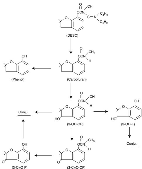
Figure 4. Metabolic pathway of dibutylaminosulfenyl carbofuran (after Umetsu et al. 1979).
