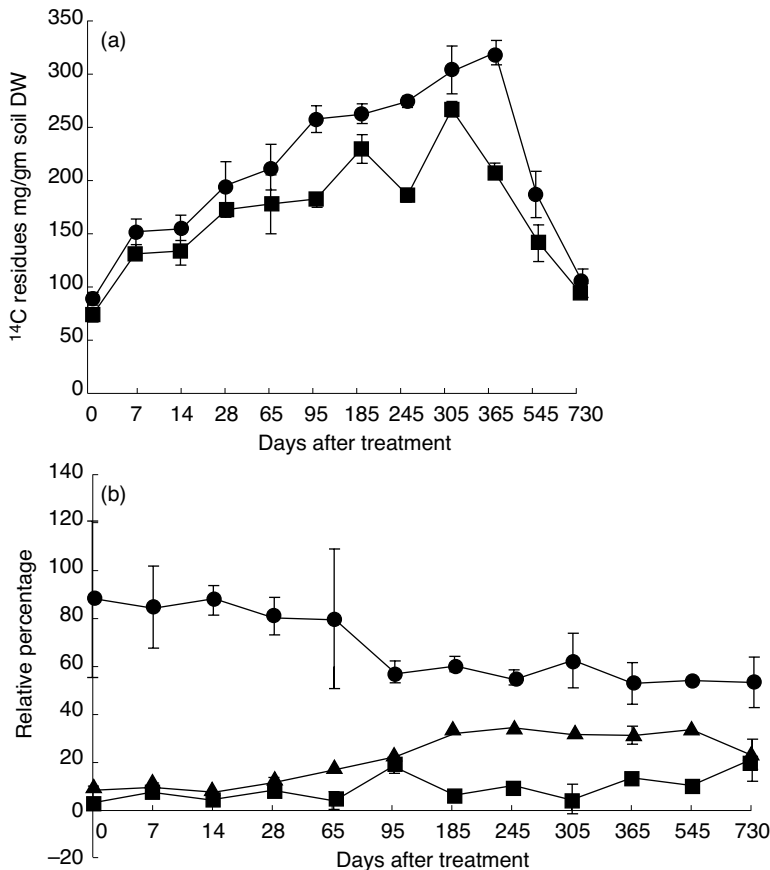
Figure 4. (a) Release of soil-bound 14 CDDDT residues by sulfuric acid: ●, initial bound residues; ■, released by sulfuric acid. (b) Composition of soil-bound residues of DDT released by sulfuric acid: ●, DDT; ■, DDD; ▲, DDE.
