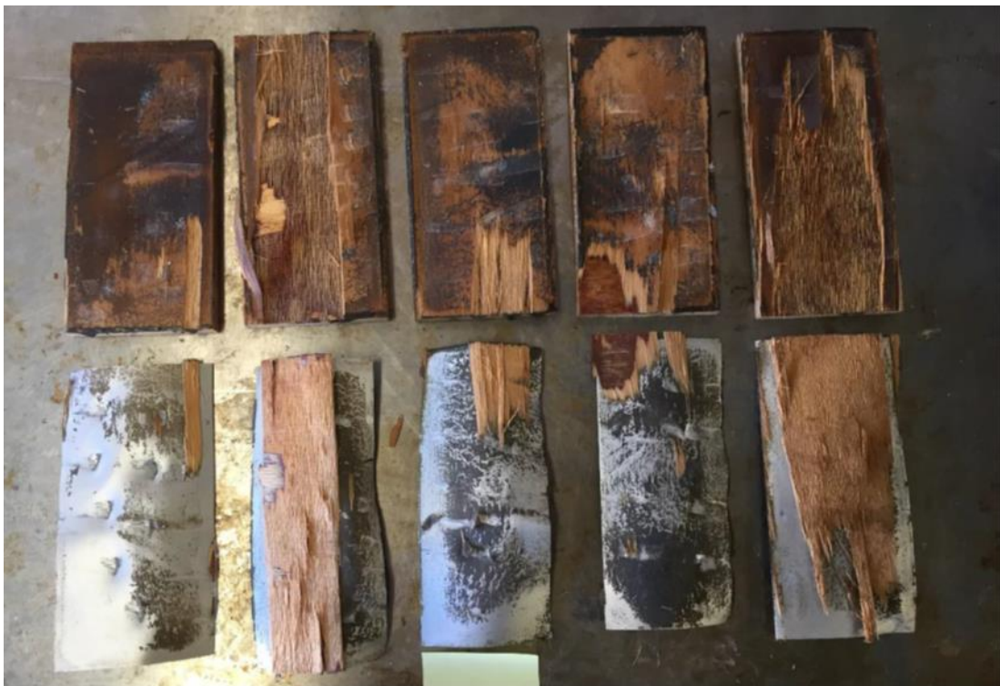
Figure 22: Aluminium overlaid plywood bond quality testing.
